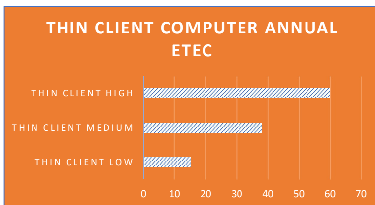
Figure 3 –Energy Star Annual Typical Energy Consumption (kWh) Range Example
